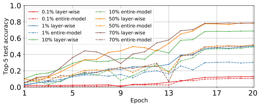
Figure 9: ImageNet top-5 test accuracy for Top k compression.
