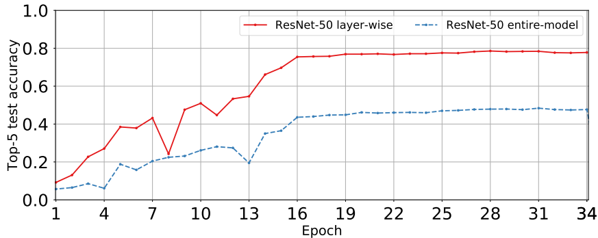
(b) ImageNet top-5 test accuracy
