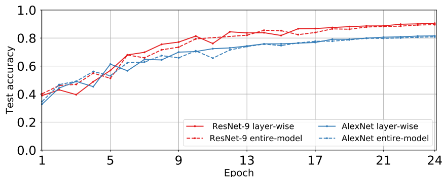
(a) CIFAR-10 test accuracy
