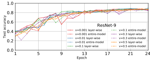
Figure 7: CIFAR-10 test accuracy for Threshold v compression.
