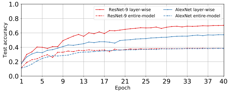
Figure 5: CIFAR-10 test accuracy for Adaptive Threshold.
