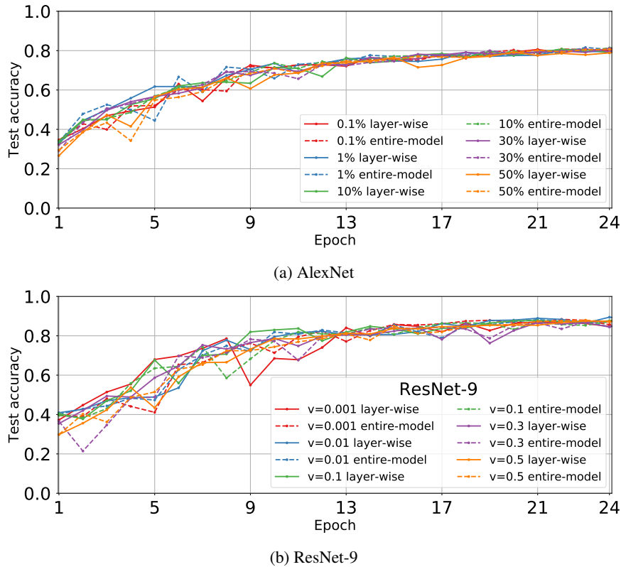
Figure 6: CIFAR-10 test accuracy for Threshold v compression.
